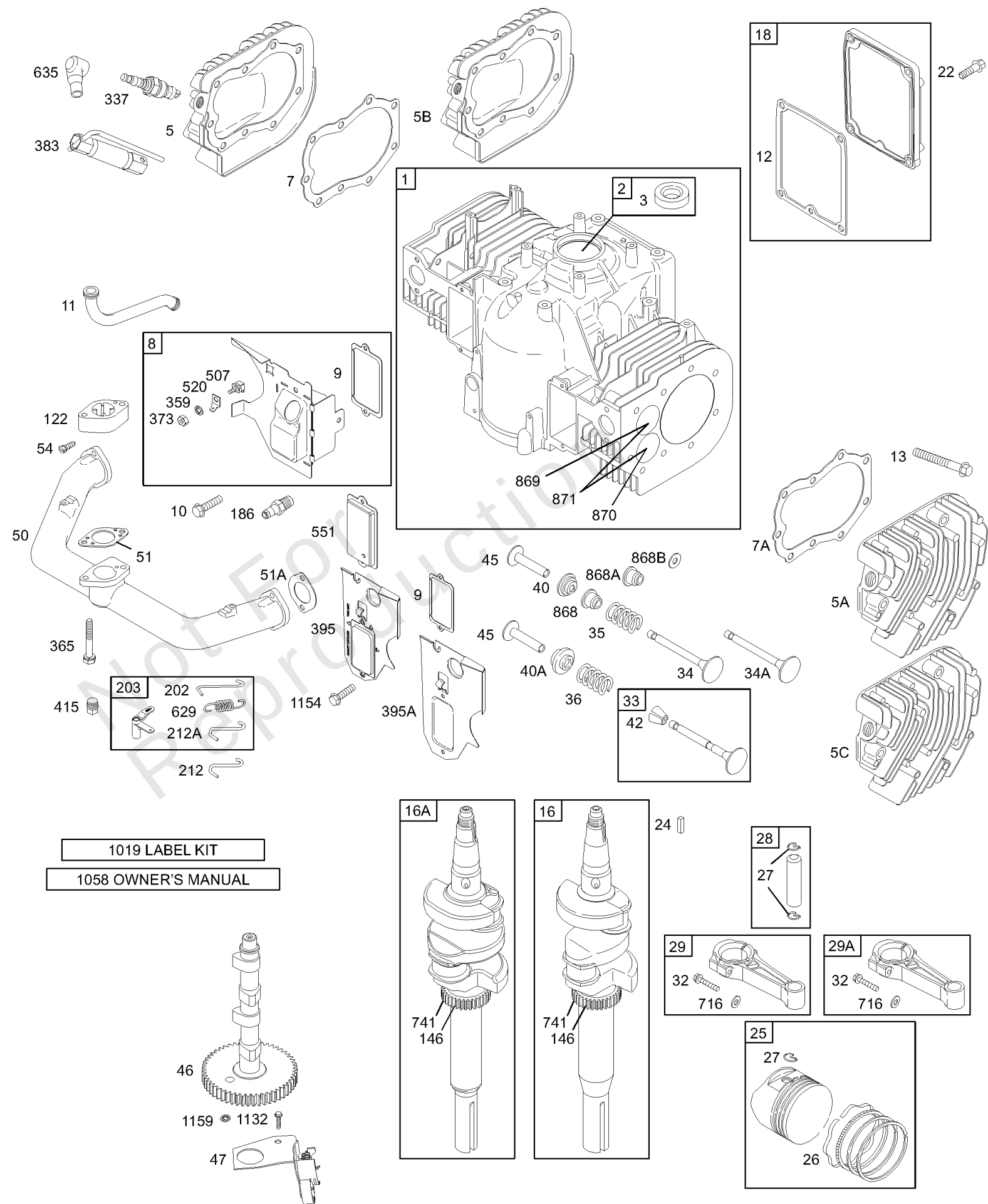
Illustrations cover a range of engines. Parts shown without corresponding text may not be used on your specific engine. Assemblies include all parts shown in frames.
